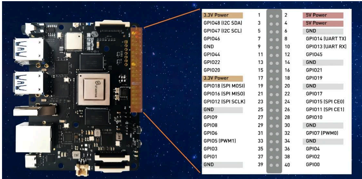
Figure 1-1 40-Pin Definition
