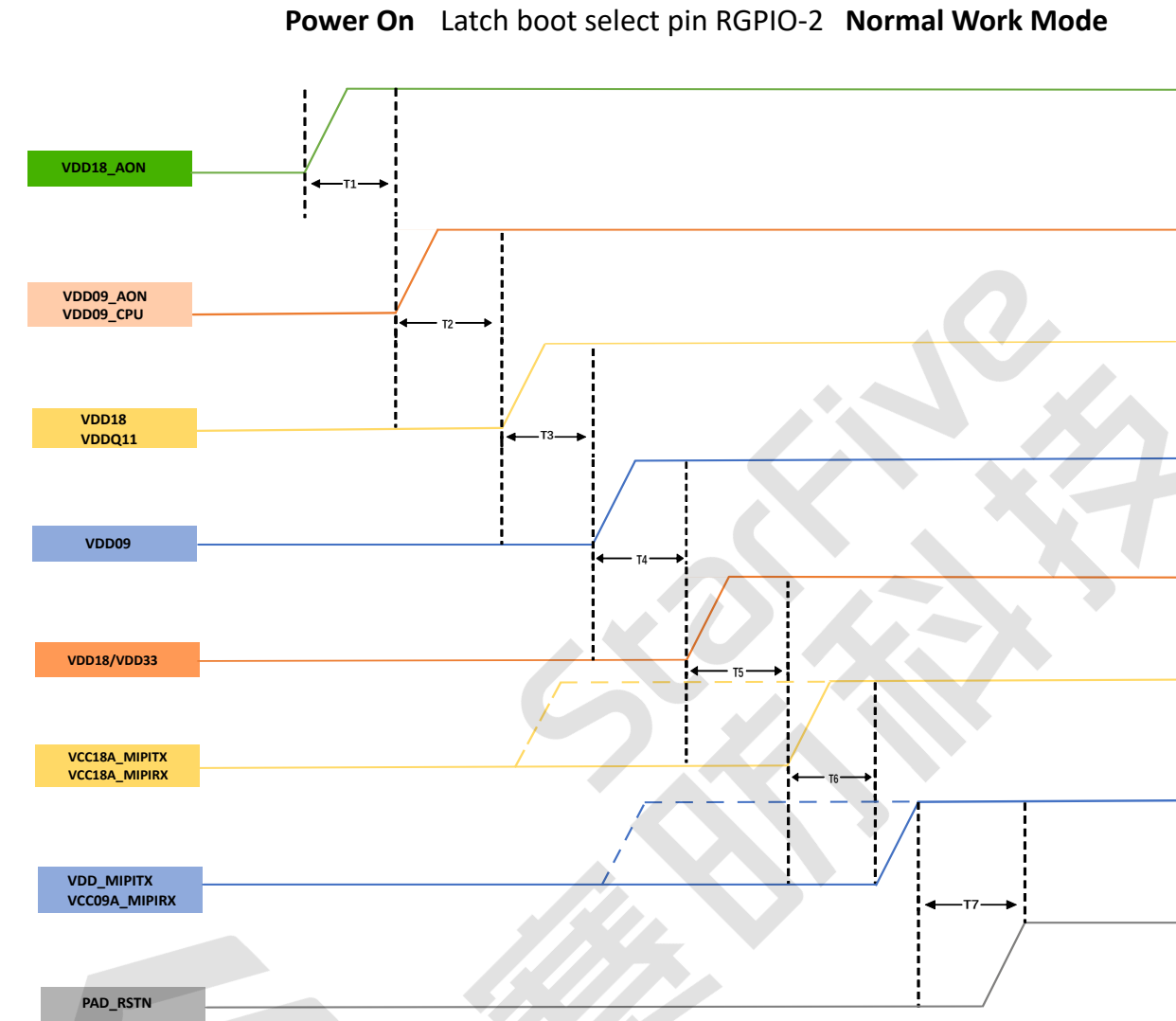
Figure 5-1 Power Up Sequence
