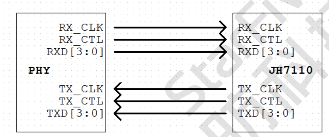
Figure 8-1 GMAC 1,000 M Only
