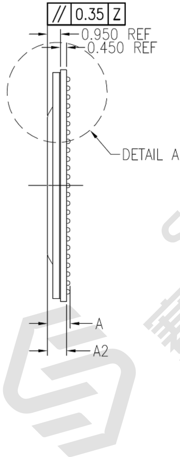
Figure 7-3 Package Side View
